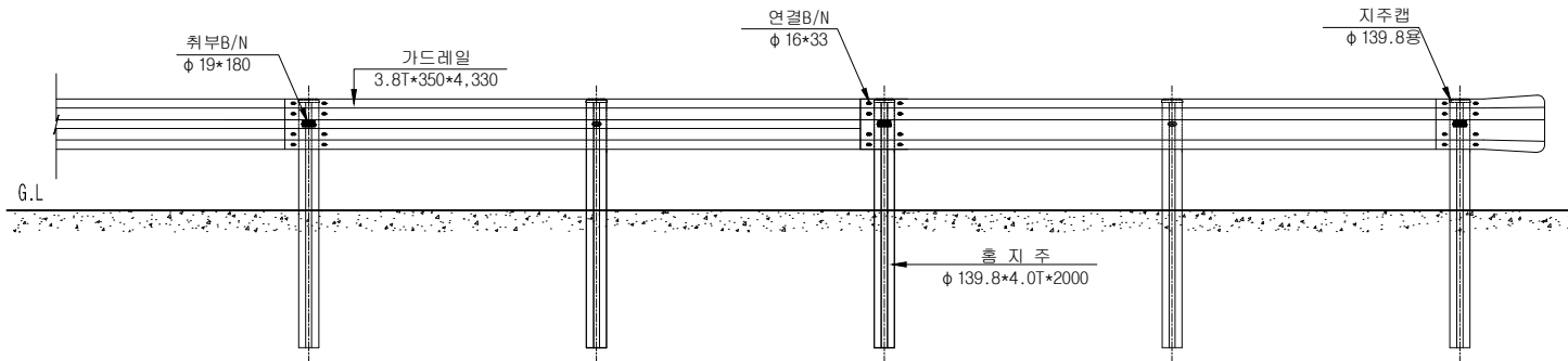
RAIL ELEVATION SCALE: NONE
