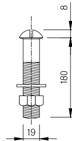
SETTING B/N ( \phi 19 \times 180 )
