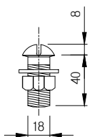
JOINTING B/N ( \phi 18 \times 50 )
