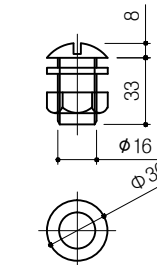
JOINTING B/N ( \phi 16 \times 33 )
