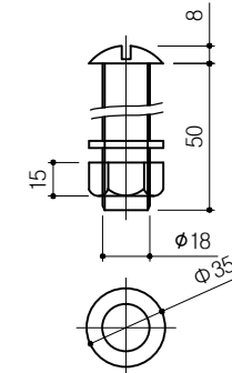
SETTING B/N ( \phi 18 \times 50 )
