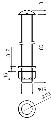
SETTING B/N ( \phi 19 \times 180 )
